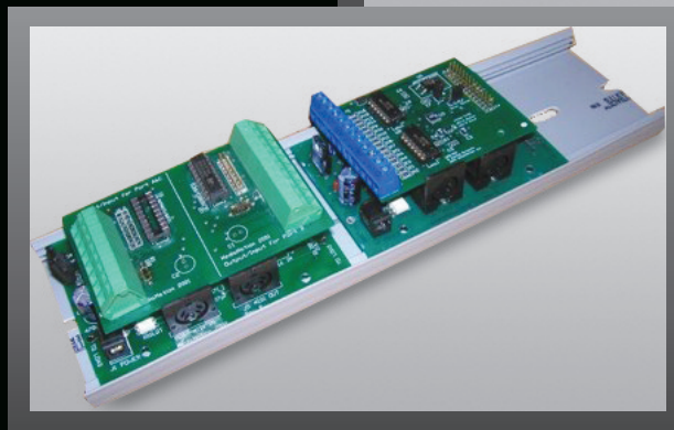
The UMB main board (above) and the UMB DO-16 and AO-8 mounted on a snap track (left).
